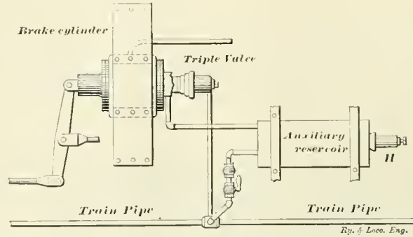
RECHARGING DEVICE ATTACHED TO PASSENGER BRAKE.
